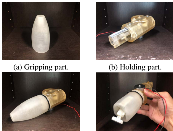
(a) Gripping part. (b) Holding part. (c) Appearance of prototype. (d) State of grasping.
