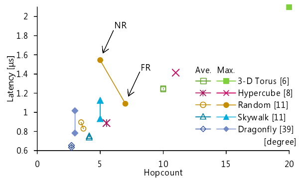
Fig. 4. Maximum and average latency vs. hop count, depending on routing scheme, in 256-cabinet, 2,048-switch networks of 60-ns switches.
