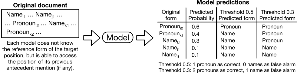
Figure 1. Toy example of how different thresholds predict pronouns and names.
