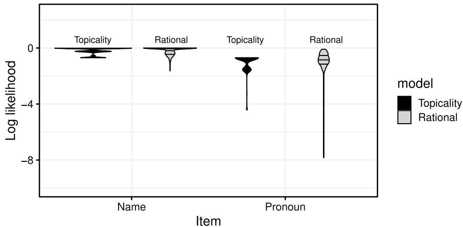
Figure 4. The distribution of log-likelihood of pronouns and proper names in each model.
