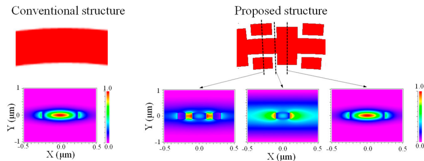
Figure 2. Electric field intensity distribution E_x of the conventional structure and the proposed structure.
