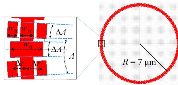
Figure 1. Design of the proposed Bragg grating structure for a micro-ring. \Delta r = 150 nm, w_b = 150 nm, w_w = 200 nm, w_0 = 500 nm, \Lambda = 5 degree, \Delta\Lambda = 2 degree.
