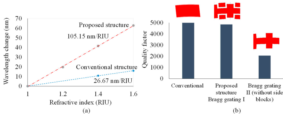
Figure 3. (a) Resonance wavelength changes due to different refractive index of the top cladding layer of the proposed structure and conventional structure. (b) Quality factor of three different structures of the conventional structure, the proposed structure (Bragg grating I), and Bragg grating II (without side blocks).
