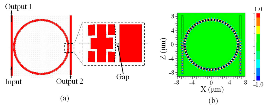
Figure 4. (a) Structure of proposed micro-ring resonator biosensor. (b) Magnetic field distribution H_y .
