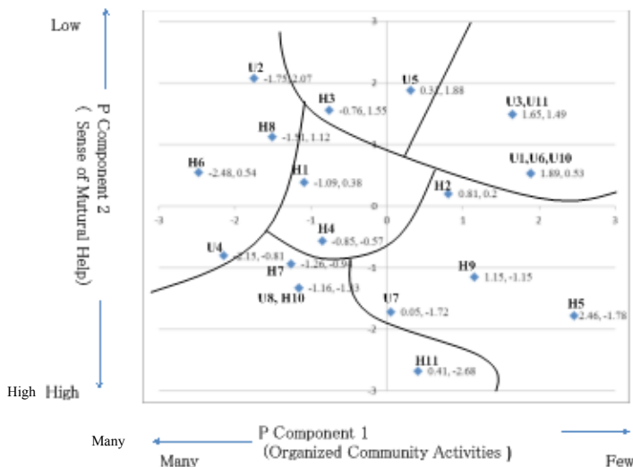
Fig.5 : Principal component analysis in combination with cluster analysis results
