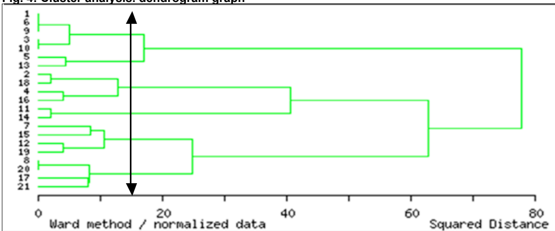
Fig. 4: Cluster analysis. dendrogram graph 7)
