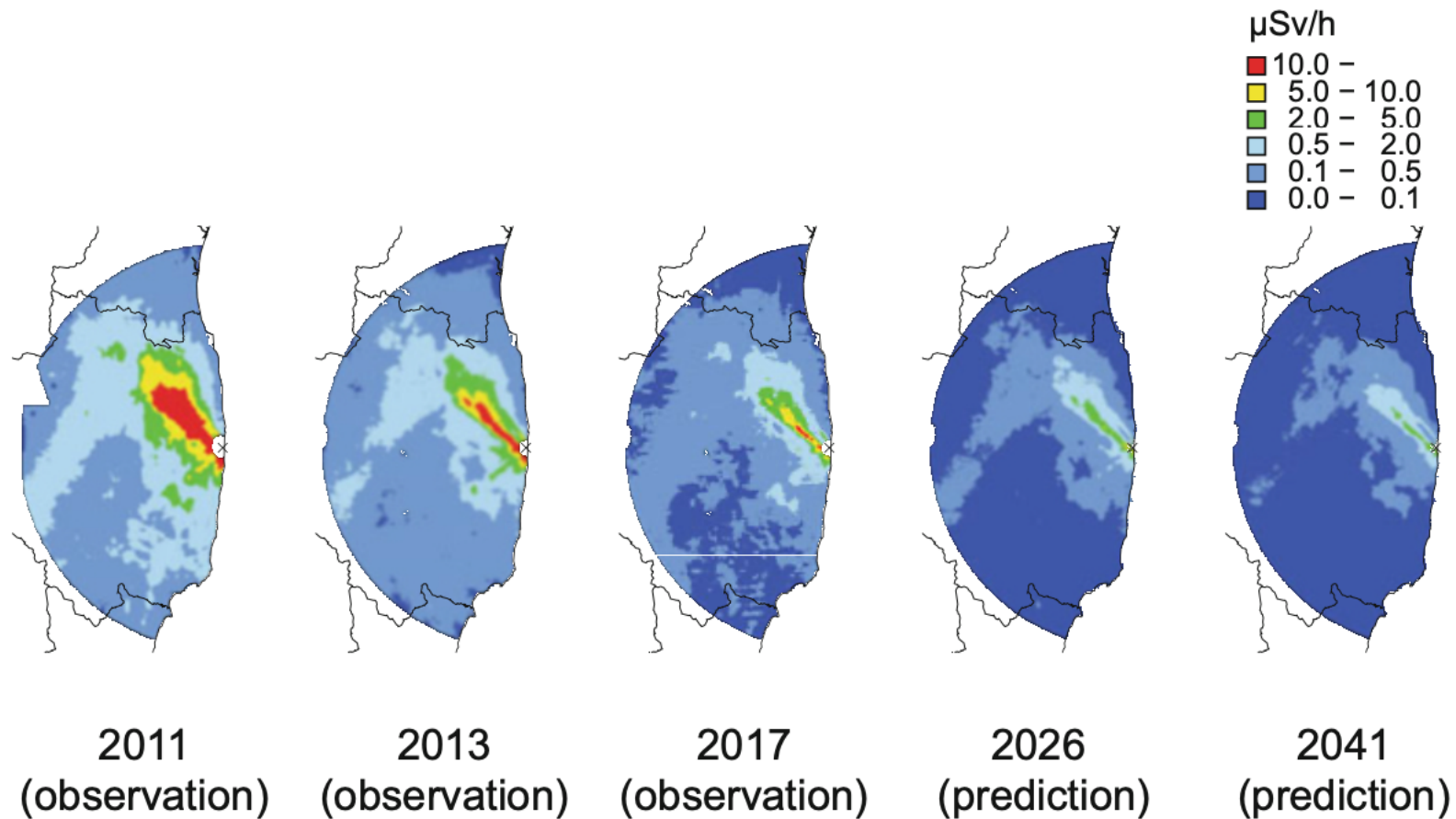
Fig. 3.19 Future predictions of air dose rate distributions within 80 km of the Fukushima Daiichi Nuclear Power Plant (Source: Data from the observation of 1st, 7th 12th Airborne Monitoring Survey [3] and the prediction of Kinase, et al. [68]; Data of prediction: Courtesy of Sakae Kinase, Japan Atomic Energy Agency)
